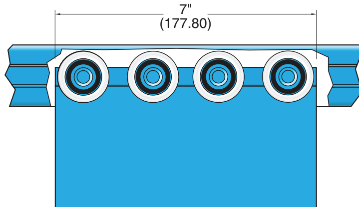
C-105-8 Hanger with C-104 track detail
