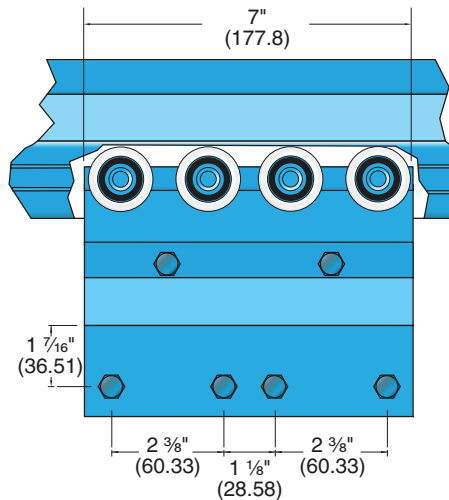
C-107-8 Hanger with C-108 Track Detail
