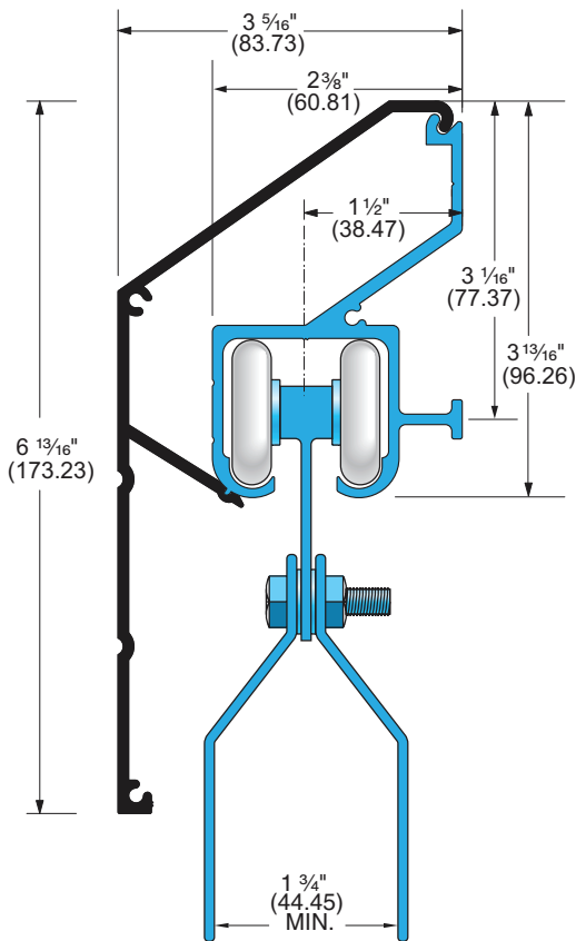
C-107-8 Hanger with C-108 Track Detail
