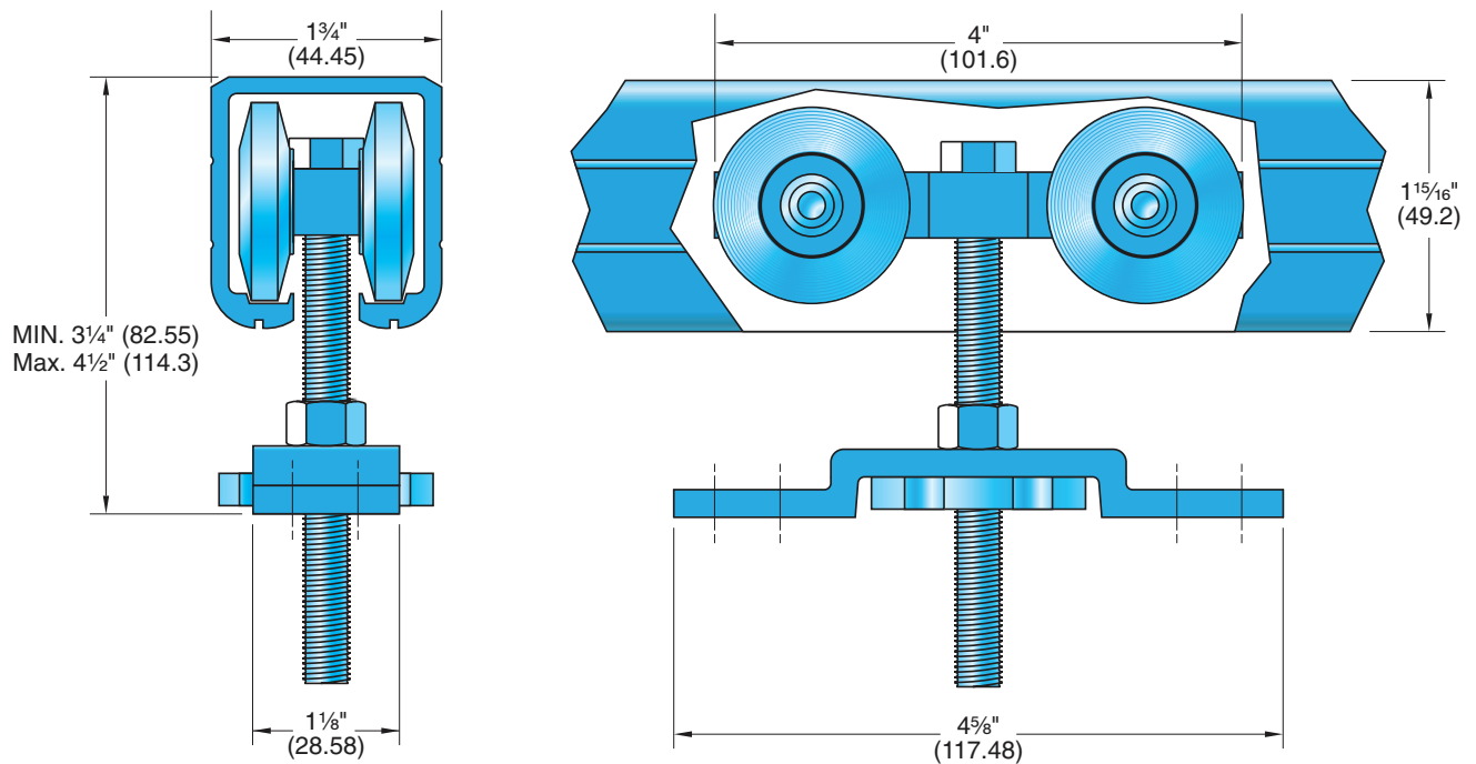
C-995 Hanger with C-204 Track Detail
