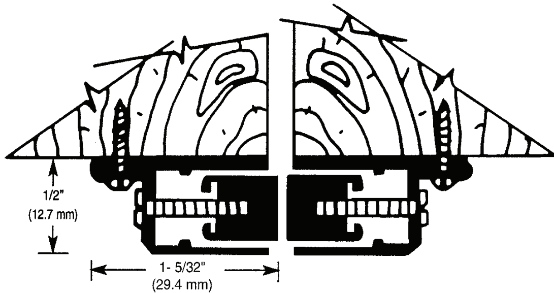
W-40 SPRING LOADED ASTRAGAL CLEAR ANODIZED EXTRUDED ALUMINUM
