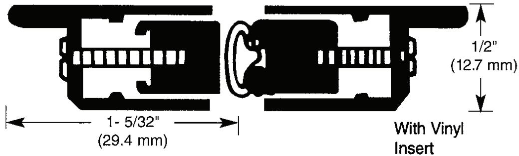
W-40V SPRING LOADED ASTRAGAL CLEAR ANODIZED EXTRUDED ALUMINUM
