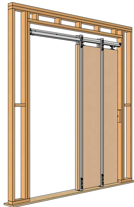
Complete Type C-B kit illustrated. Framing by others.
