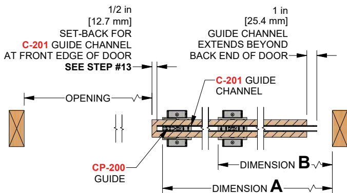
Opened position
