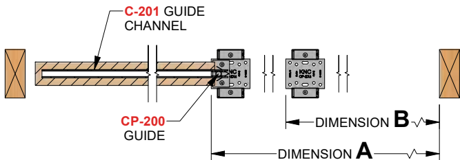
Closed position
