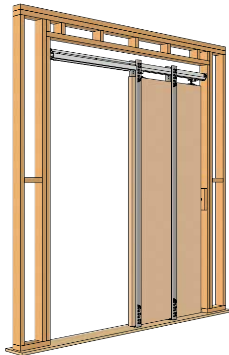
Complete Type C-W kit illustrated. Framing by others.
