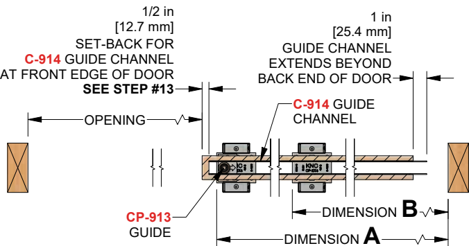
Opened position
