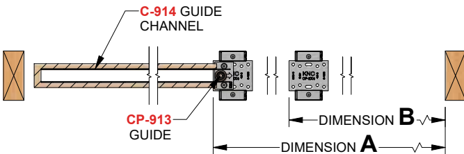
Closed position
