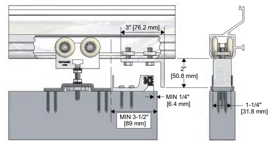
(CAS-2 IS SHOWN WITH C-108 TRACK AND C-911 HANGER)
