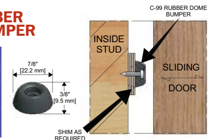
SHIMS REQUIRED
