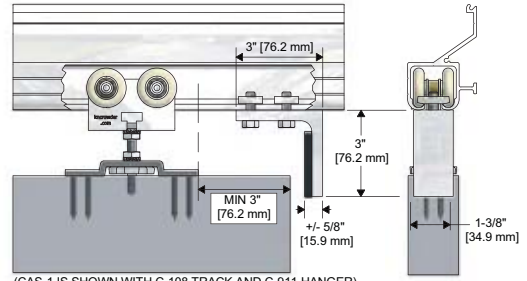
(CAS-1 IS SHOWN WITH C-108 TRACK AND C-911 HANGER)
