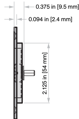
C-60RT Round Thumb Turn Flush Pull
