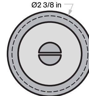
C-60RE Round Emergency Release Coin Turn Flush Pull
