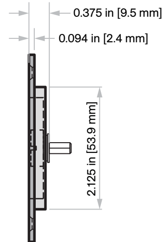
C-60RE Round Flush Pull with Emergency Coin Turn
