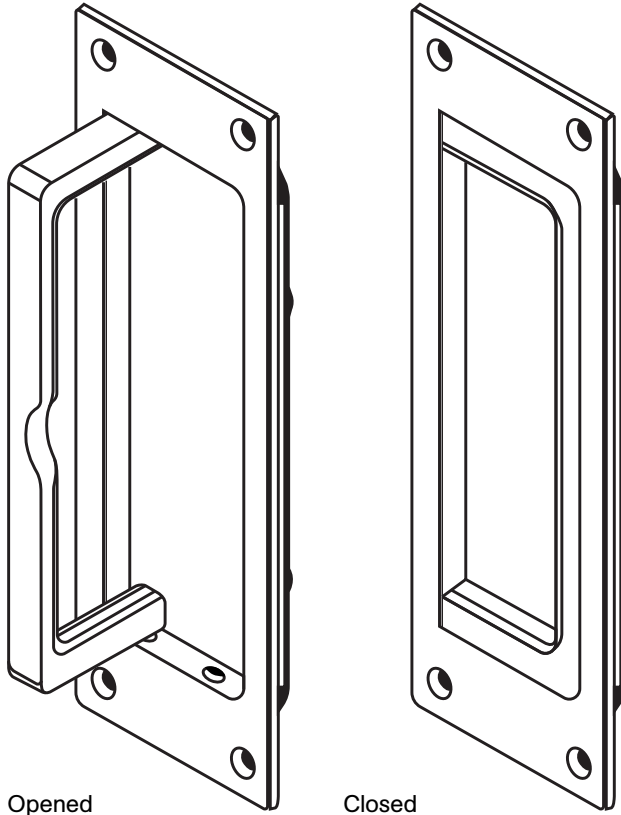
C-90BH Swing-Out Handle Flush Pull
