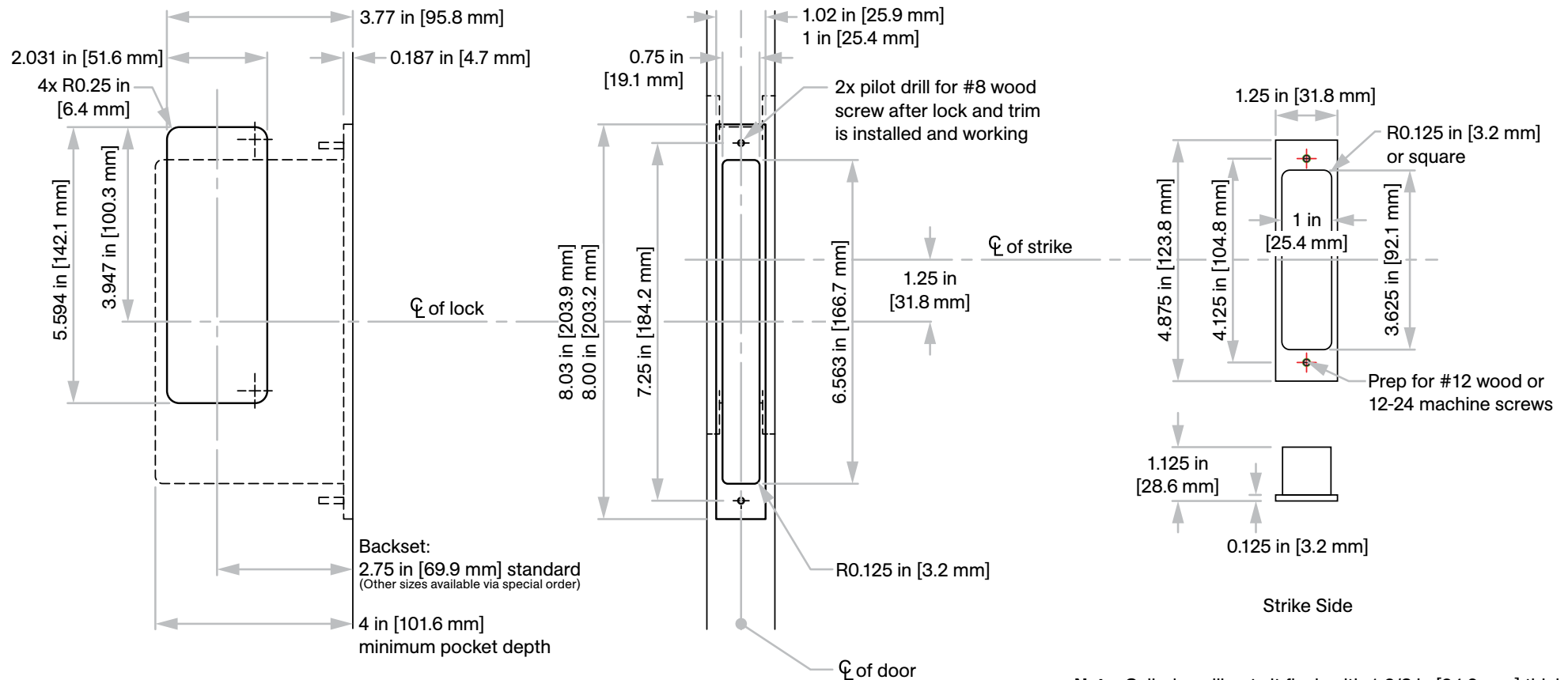
C-90OI Occupancy Indicator with Coin Turn Flush Pull
