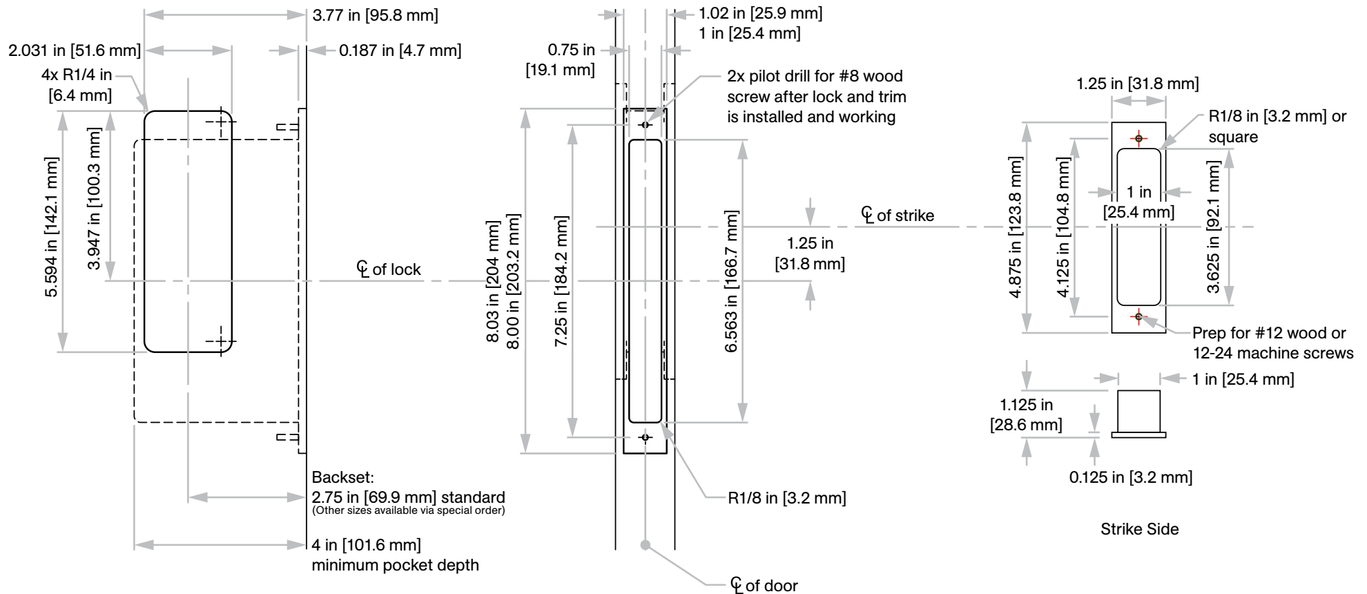
C-90TS Thumb Slide Flush Pull with Short Spindle
