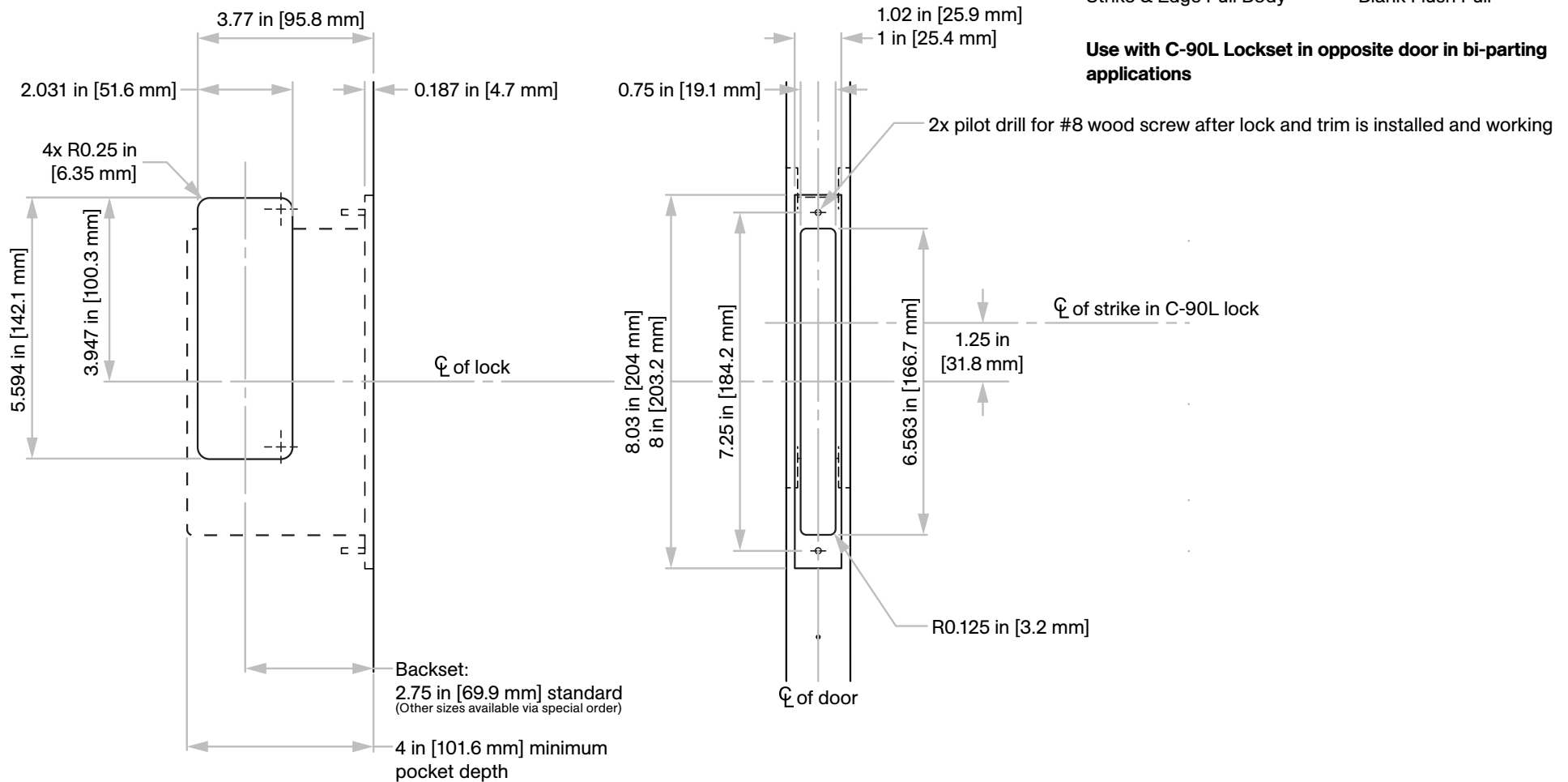
C-90S Strike & Edge Pull Body
