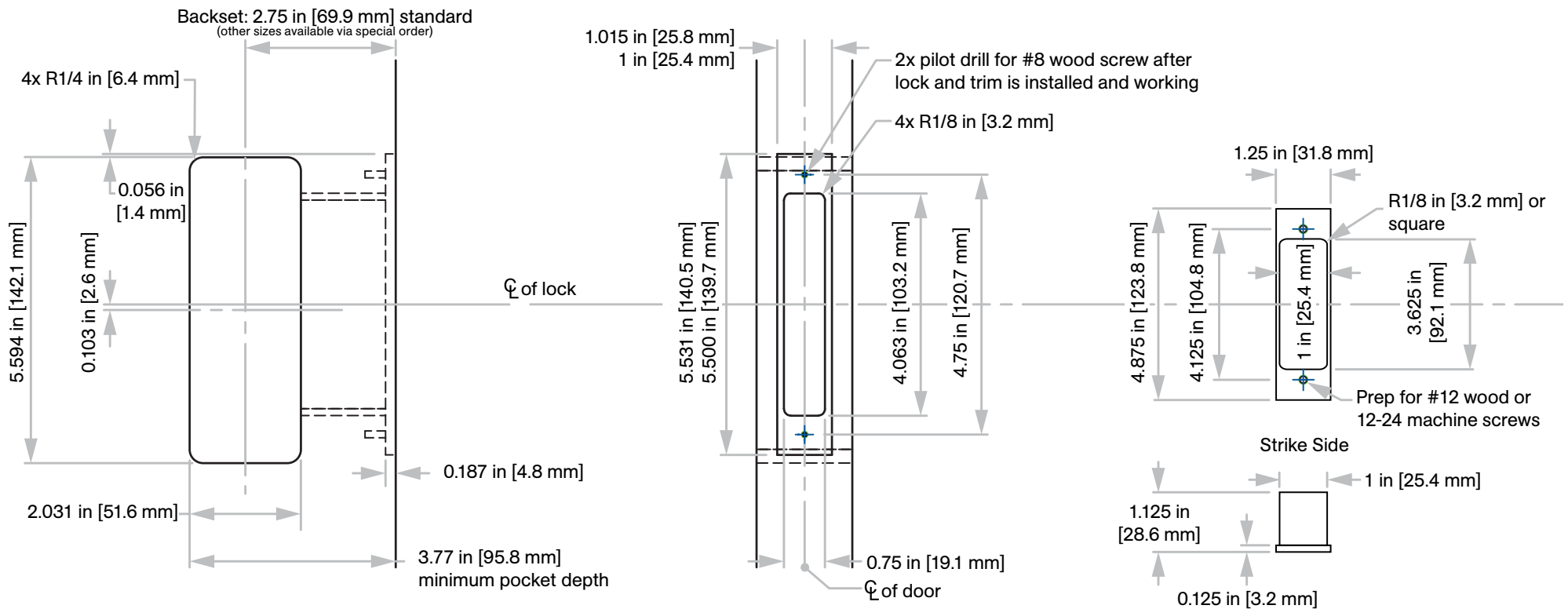
C-90E Emergency Release Flip Cover Flush Pull
