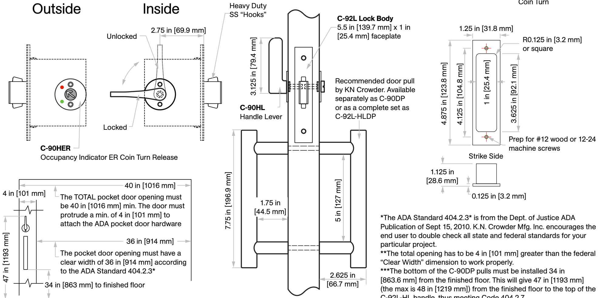
C-92L Lock Body
