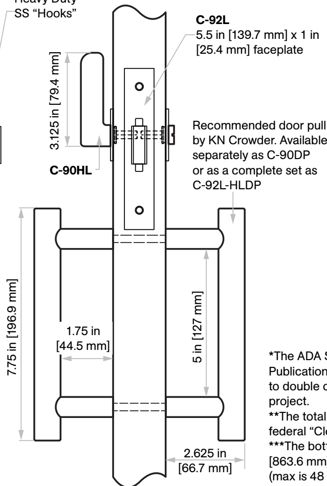
C-92L Lock Body
