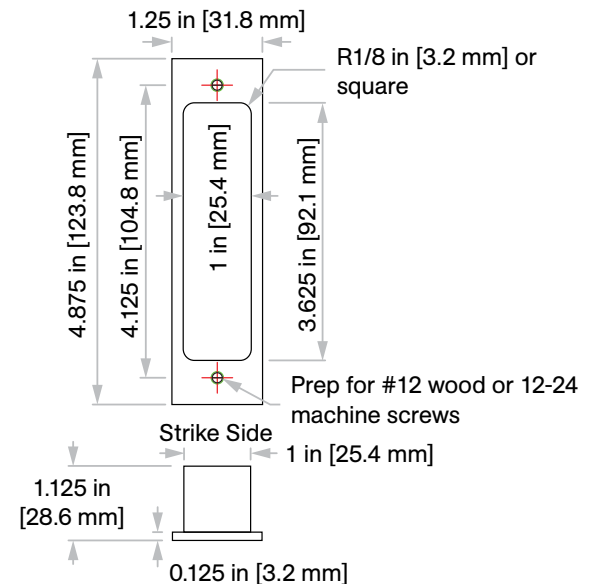
C-90HER / C-90HER-138 Occupancy Indicator with Coin Turn Emergency Release
