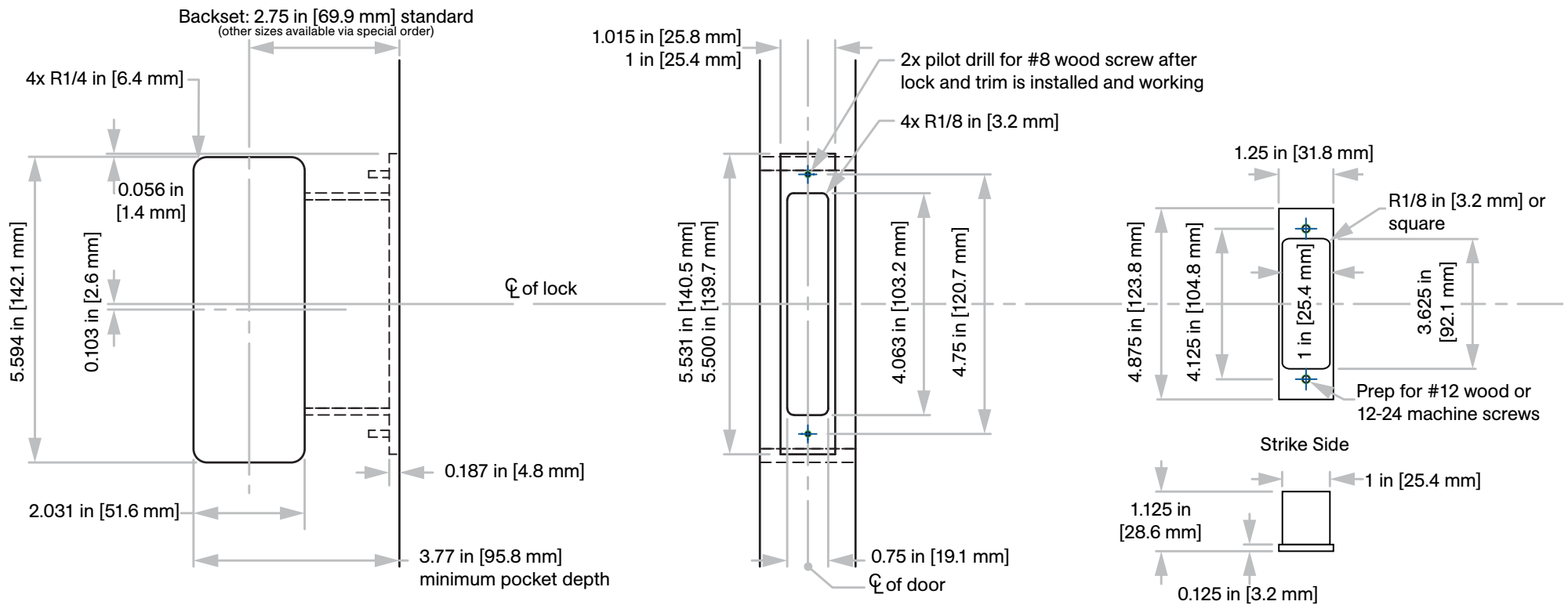
C-90TS Thumb Slide Flush Pull with Short Spindle
