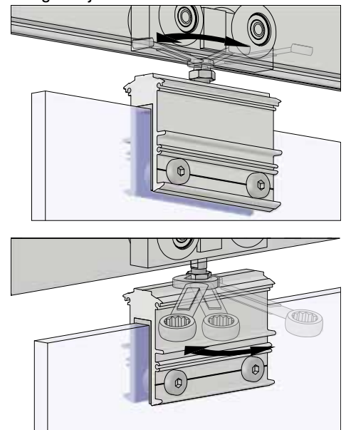
Hanger adjustment view
