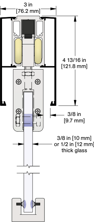
Optional CC-940 Snap-on Fascia, illustrated as solid black profile
