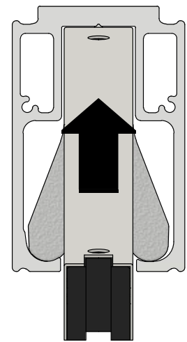
End view
