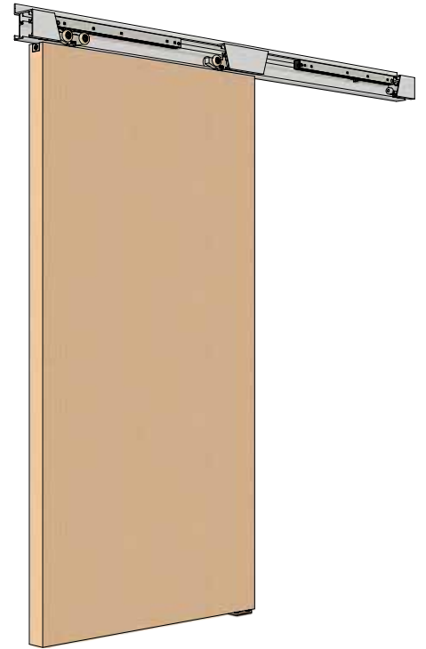
Complete CCS-410-W kit illustrated. Cut-outs in track to expose components.
