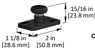
C-913 FLOOR GUIDE (1)
