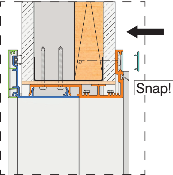
View from front wall, Strike Jamb side
