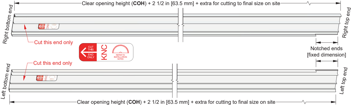
CS-25C Casing Cover Verticals (1 right and 1 left)
