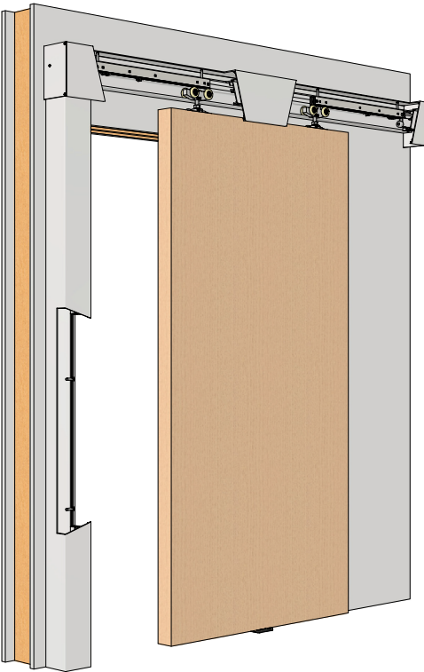
Complete Crowder Strike with CCSF-493 kit illustrated. Framing by others.
