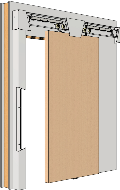
Complete Crowder Strike with CCSF-993 kit illustrated. Framing by others.
