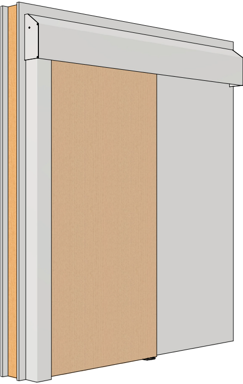
Complete Crowder Strike with CCSSF-993 kit illustrated. Framing by others.
