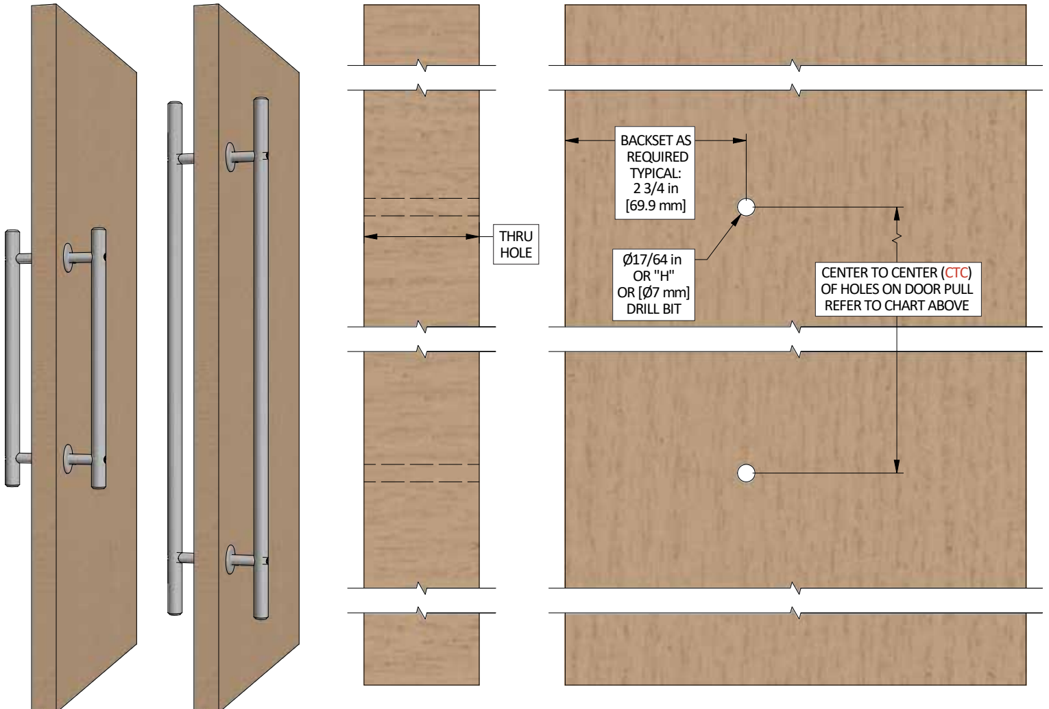
CRT-DP18 (18 in [457 mm]) SHOWN ON LEFT CRT-DP36 (36 in [914 mm]) SHOWN ON RIGHT
