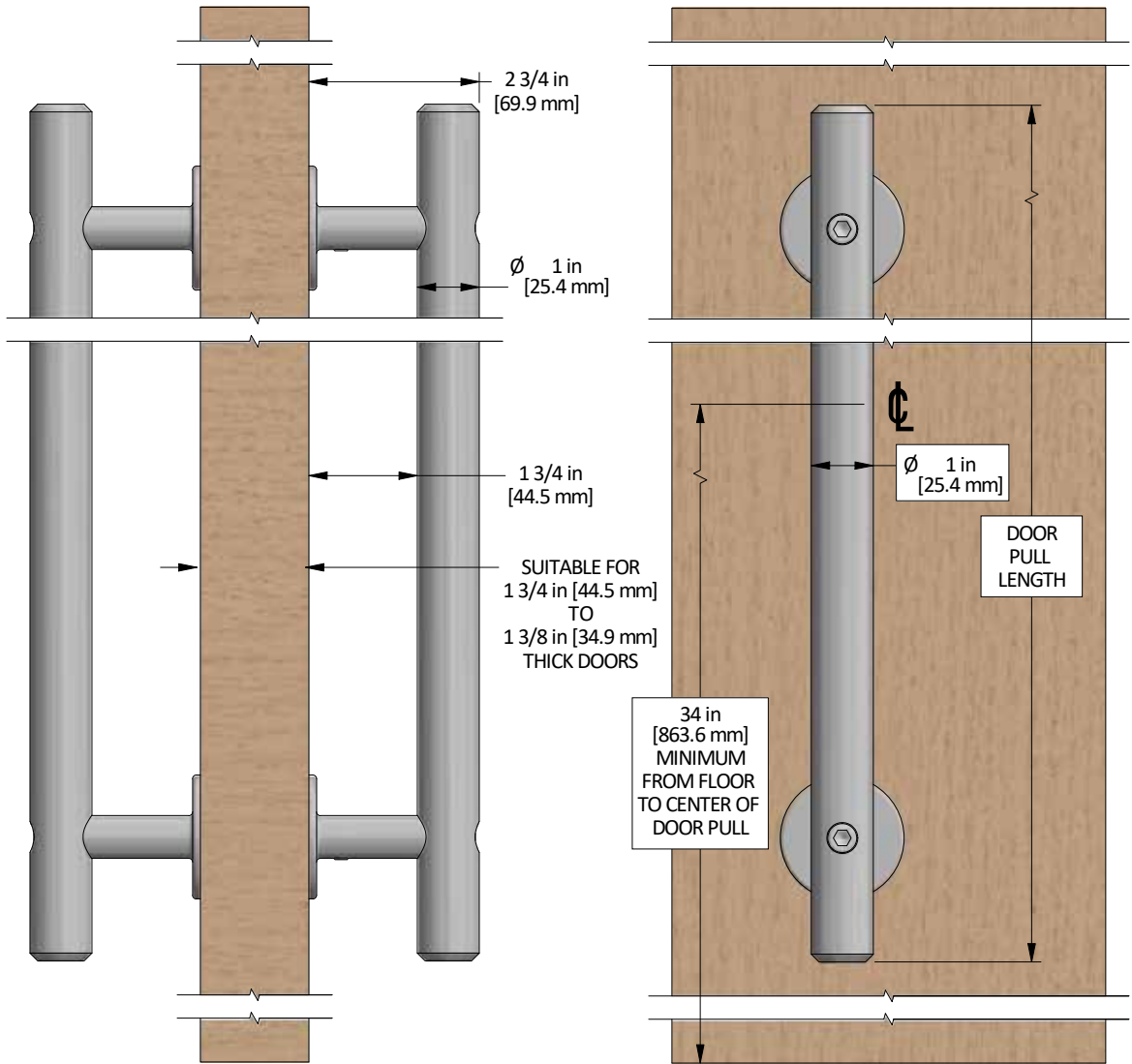
CRT-DP18 (18 in [457 mm]) SHOWN ON LEFT CRT-DP36 (36 in [914 mm]) SHOWN ON RIGHT
