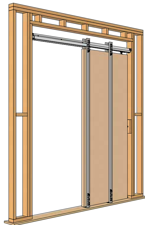
Complete Type B-B kit illustrated. Framing by others.
