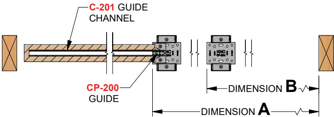
Closed position
