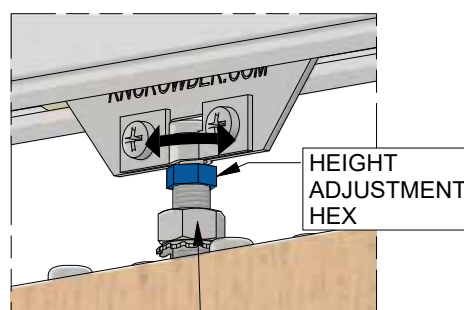
LOCKING NUT
