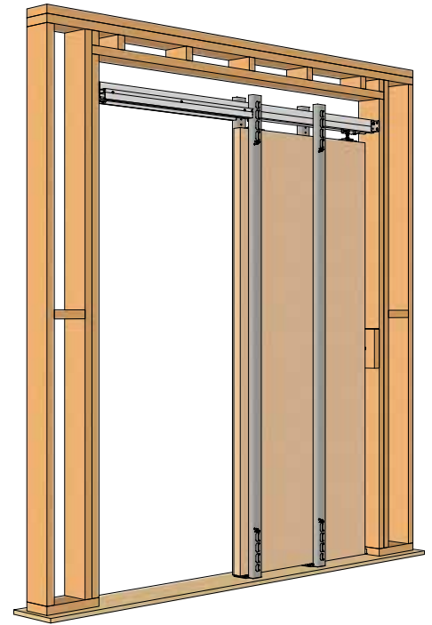
Complete Type C-B-2X6 kit illustrated. Framing by others..
