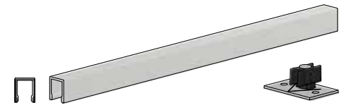
Complete Type C-B-2X6 kit illustrated. Framing by others..
