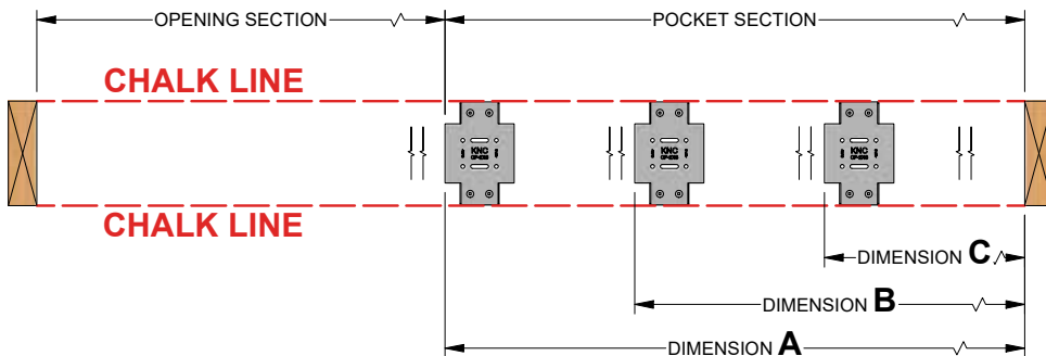
-EXW4 (extra width) Plan View For doors 37 in [940 mm] to 48 in [1219 mm] wide
