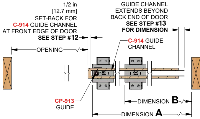
Opened position
