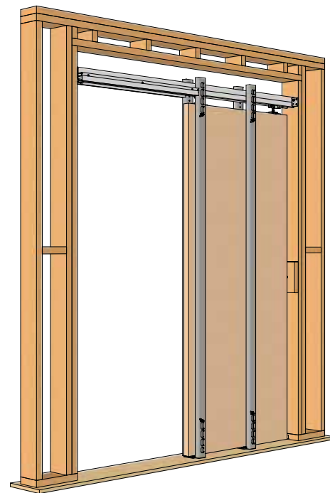
Complete Type C-W-2X6 kit illustrated. Framing by others..
