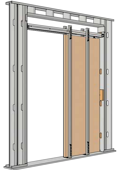
Complete Type CC-NRB-6MS kit illustrated. Framing by others.
